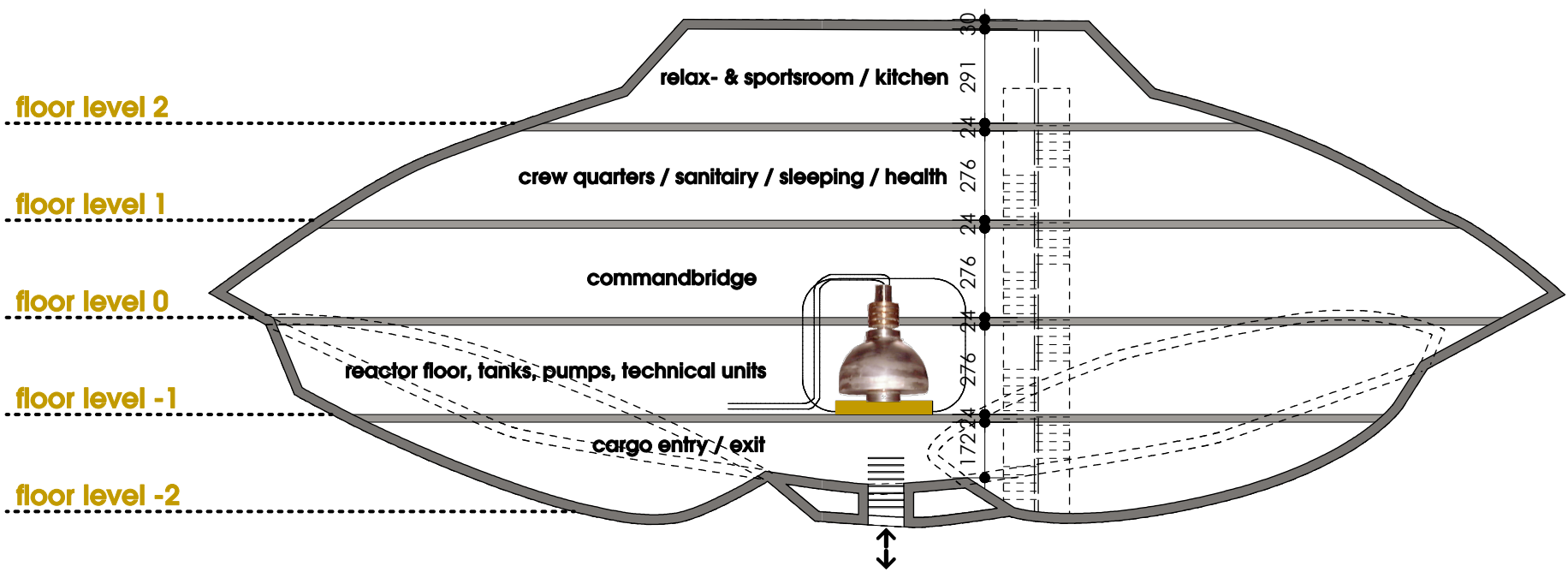
section: scale 1/200
