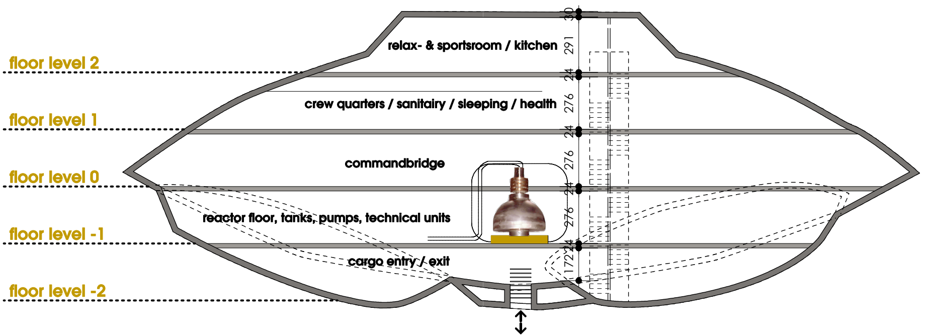
section: scale 1/200
